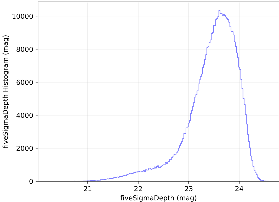
too_ignore_100_4v3.4_10yrs WFD i band: fiveSigmaDepth Histogram
