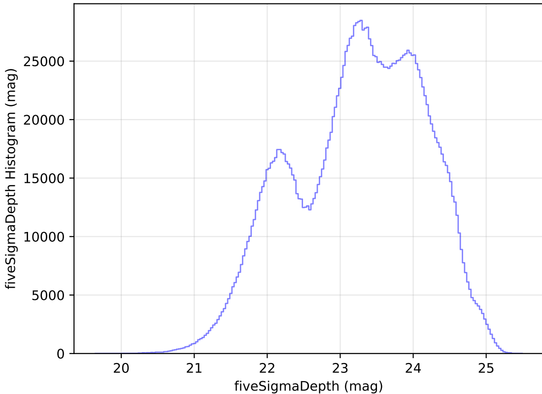
too_ignore_100_4v3.4_10yrs WFD all bands: fiveSigmaDepth Histogram
