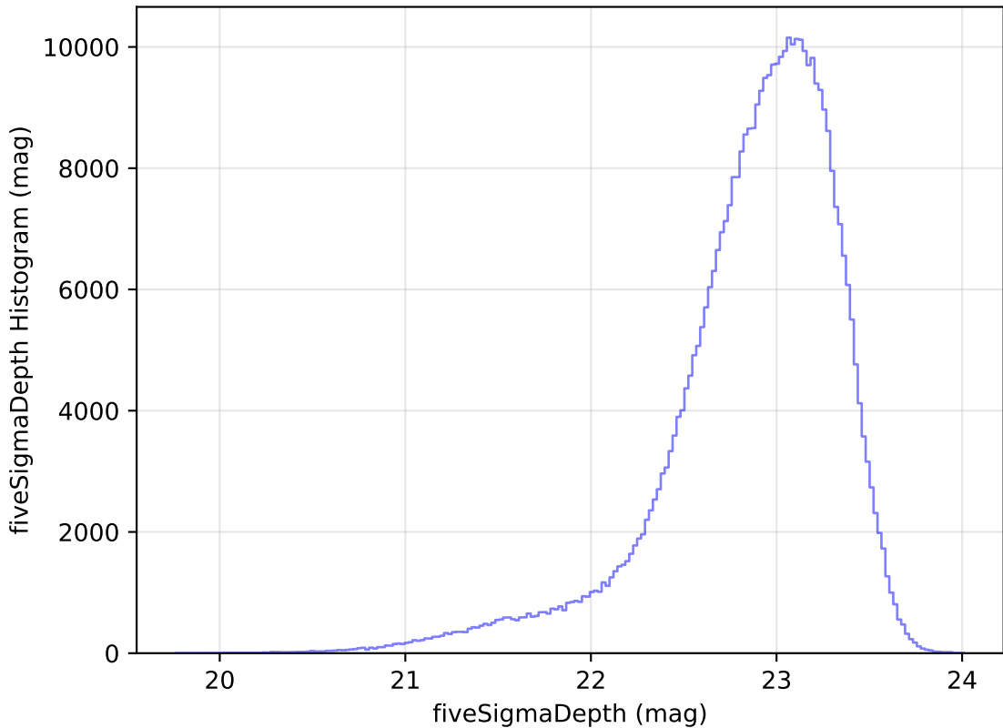
too_ignore_100_4v3.4_10yrs All sky z band: fiveSigmaDepth Histogram
