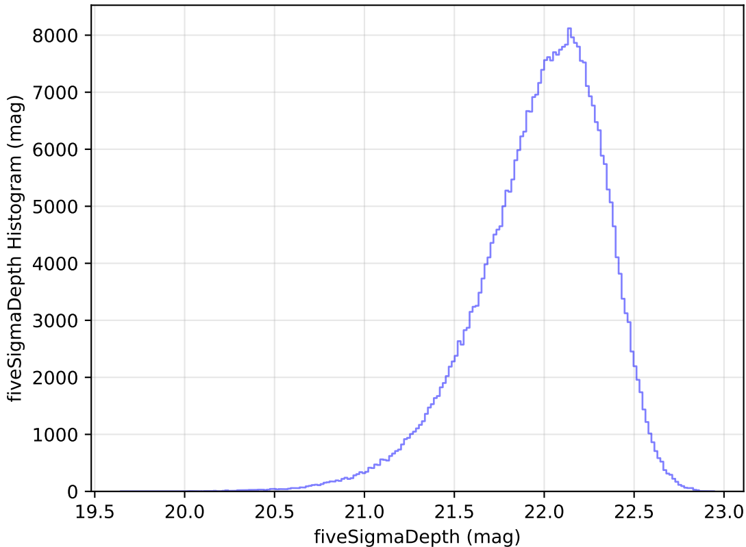
too_ignore_100_4v3.4_10yrs All sky y band: fiveSigmaDepth Histogram
