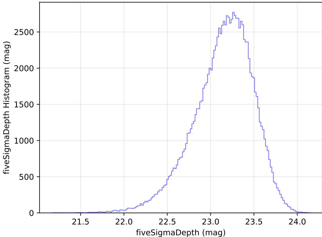
too_ignore_100_4v3.4_10yrs All sky u band: fiveSigmaDepth Histogram
