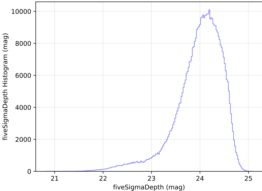
too_ignore_100_4v3.4_10yrs All sky r band: fiveSigmaDepth Histogram
