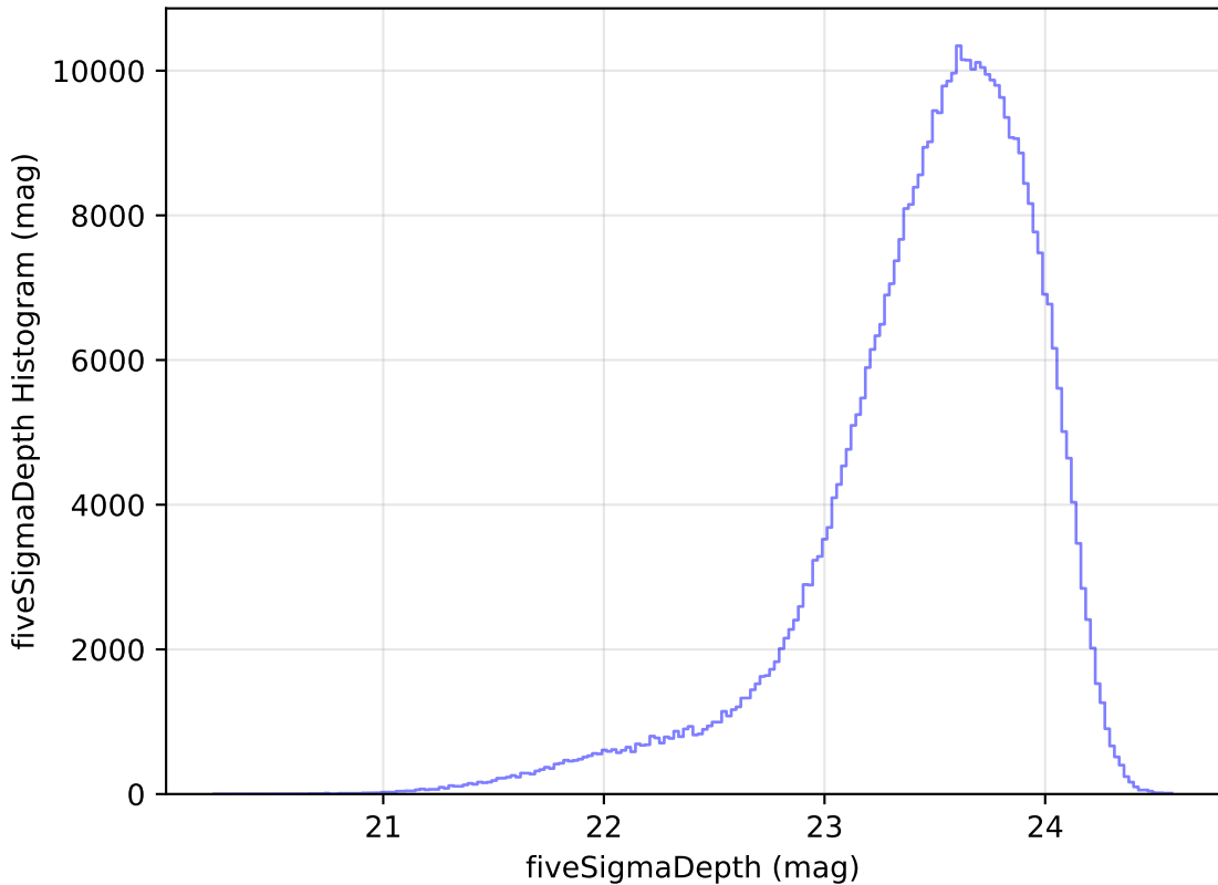
too_ignore_100_4v3.4_10yrs All sky i band: fiveSigmaDepth Histogram
