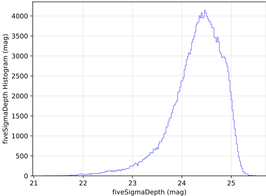
too_ignore_100_4v3.4_10yrs All sky g band: fiveSigmaDepth Histogram
