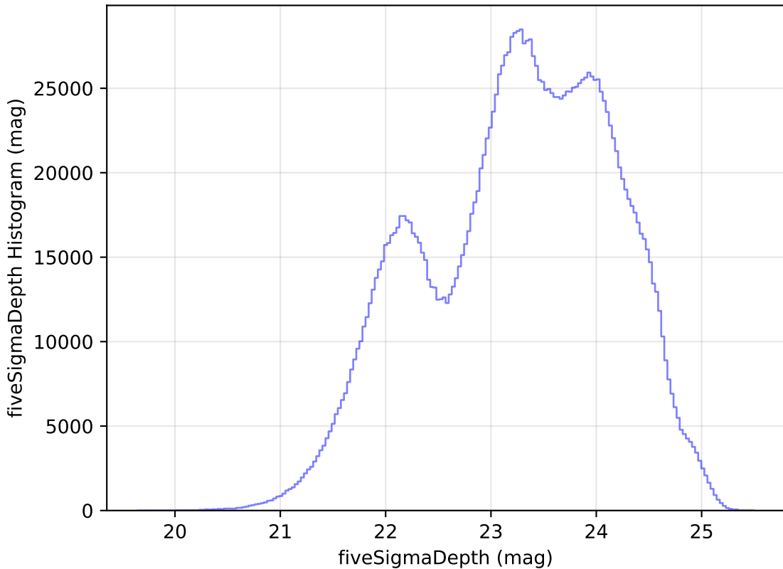
too_ignore_100_4v3.4_10yrs All sky all bands: fiveSigmaDepth Histogram
