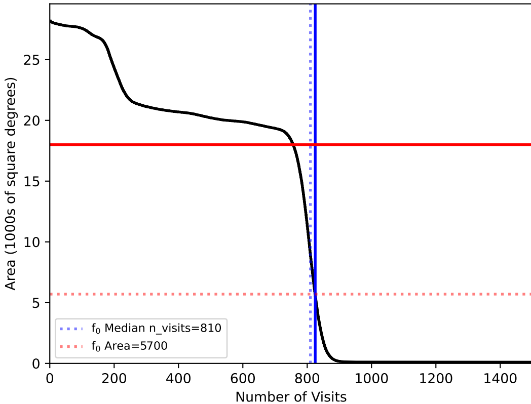
too_ignore_100_4v3.4_10yrs All sky: f0
