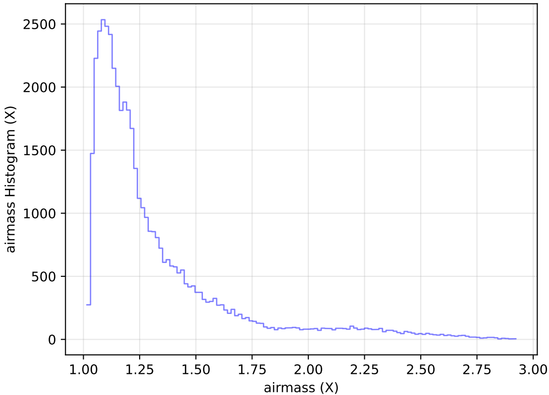
too_ignore_100_4v3.4_10yrs Yr 1 z band: airmass Histogram
