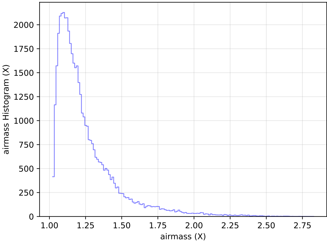
too_ignore_100_4v3.4_10yrs Yr 1 y band: airmass Histogram
