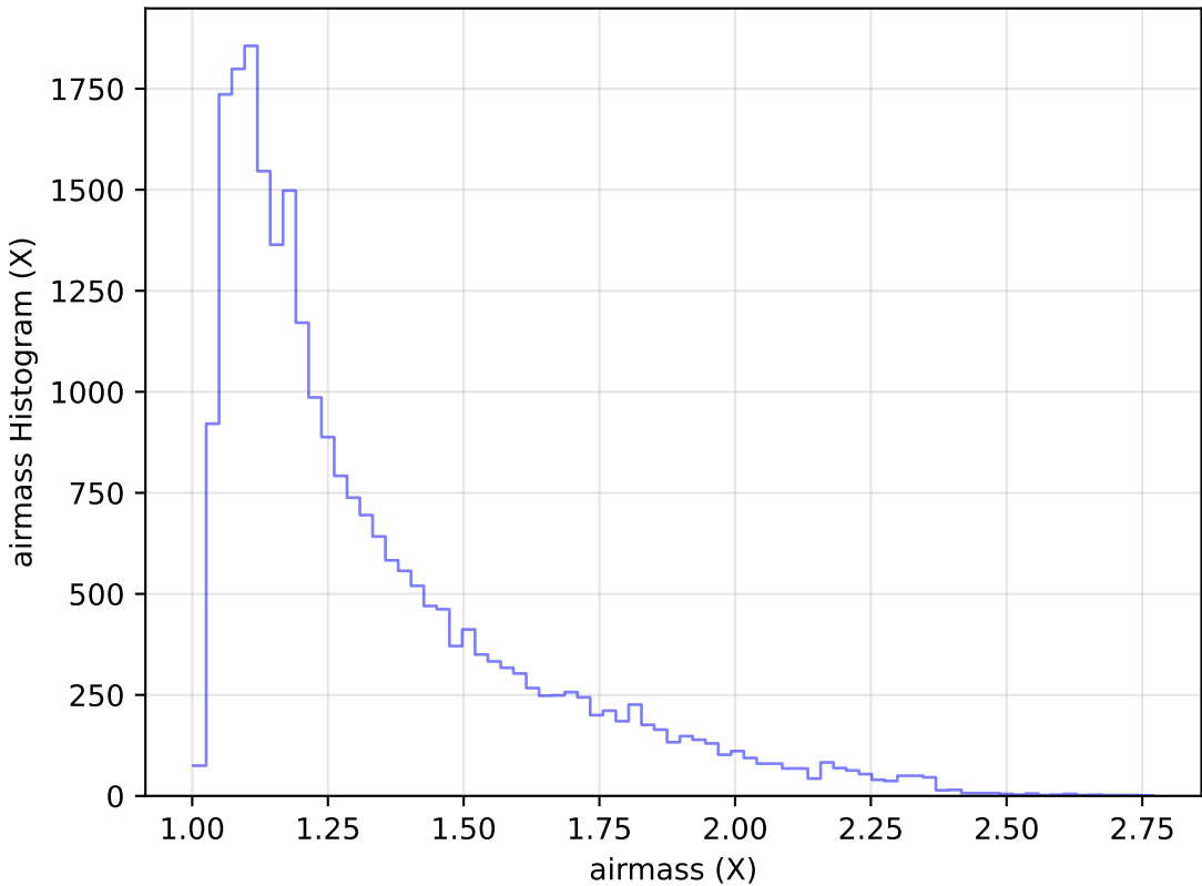
too_ignore_100_4v3.4_10yrs Yr 1 g band: airmass Histogram
