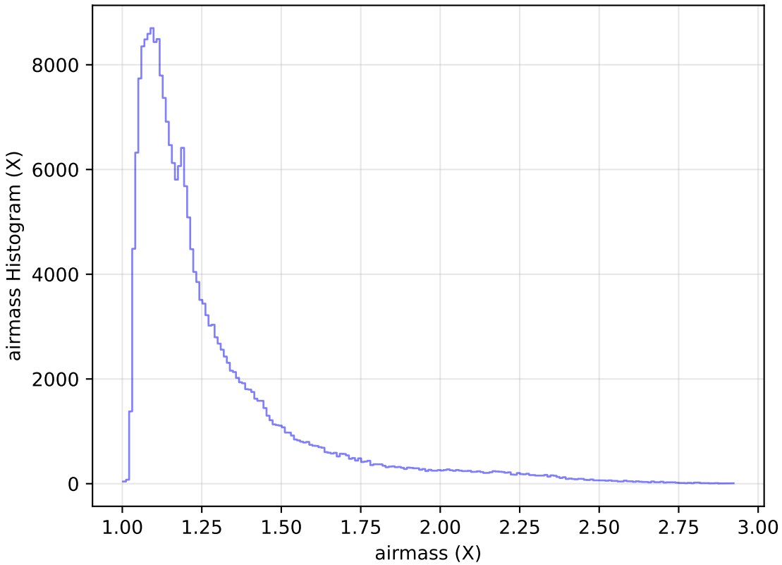
too_ignore_100_4v3.4_10yrs Yr 1 all bands: airmass Histogram
