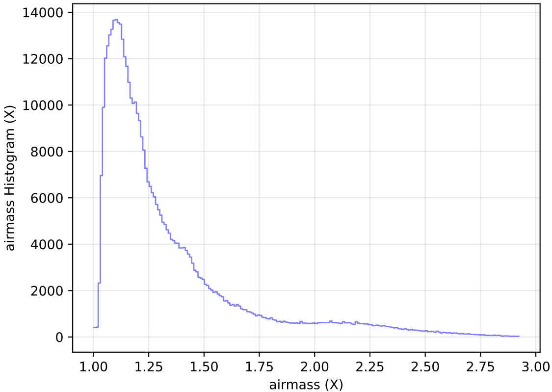
too_ignore_100_4v3.4_10yrs WFD z band: airmass Histogram
