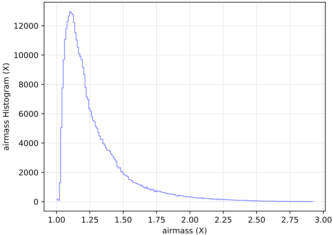
too_ignore_100_4v3.4_10yrs WFD y band: airmass Histogram
