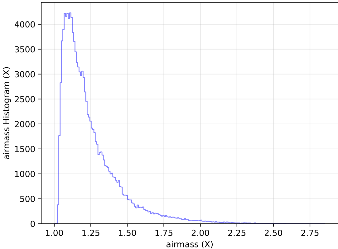
too_ignore_100_4v3.4_10yrs WFD u band: airmass Histogram
