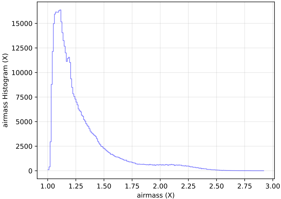
too_ignore_100_4v3.4_10yrs WFD r band: airmass Histogram
