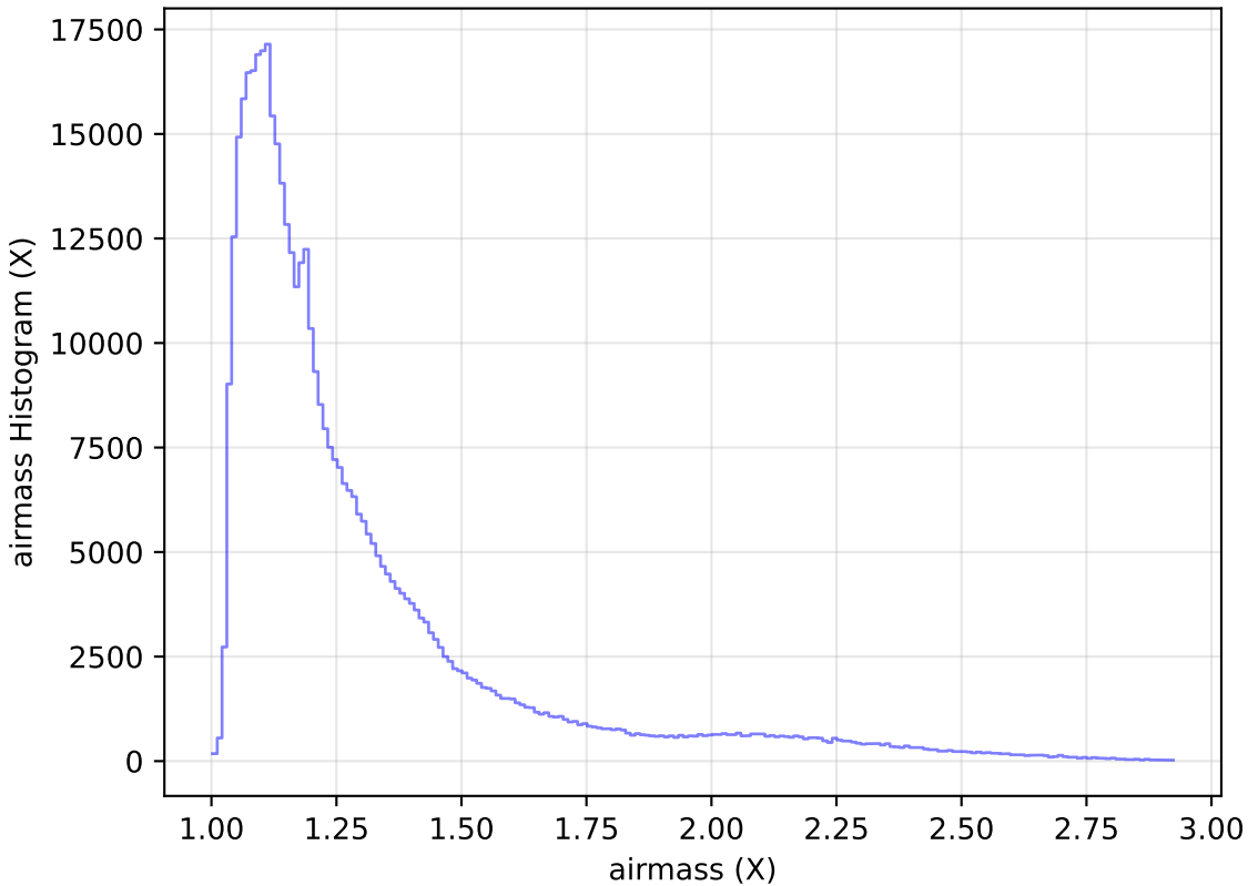
too_ignore_100_4v3.4_10yrs WFD i band: airmass Histogram
