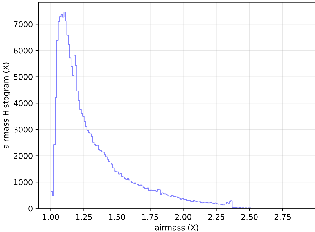
too_ignore_100_4v3.4_10yrs WFD g band: airmass Histogram
