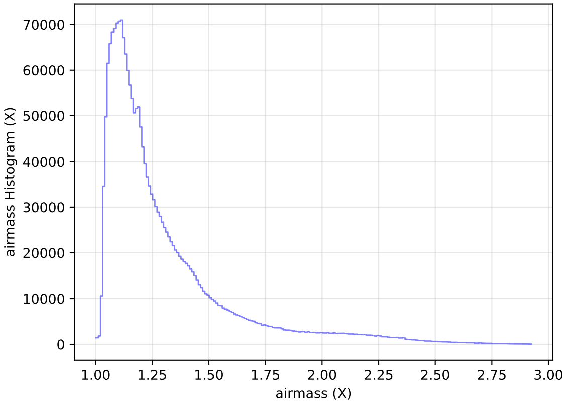
too_ignore_100_4v3.4_10yrs WFD all bands: airmass Histogram
