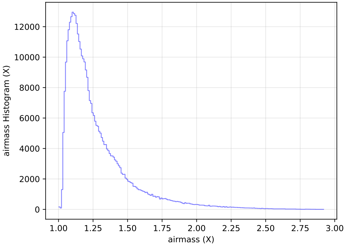
too_ignore_100_4v3.4_10yrs All sky y band: airmass Histogram
