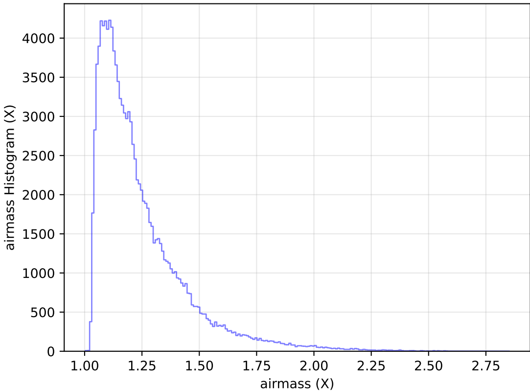
too_ignore_100_4v3.4_10yrs All sky u band: airmass Histogram
