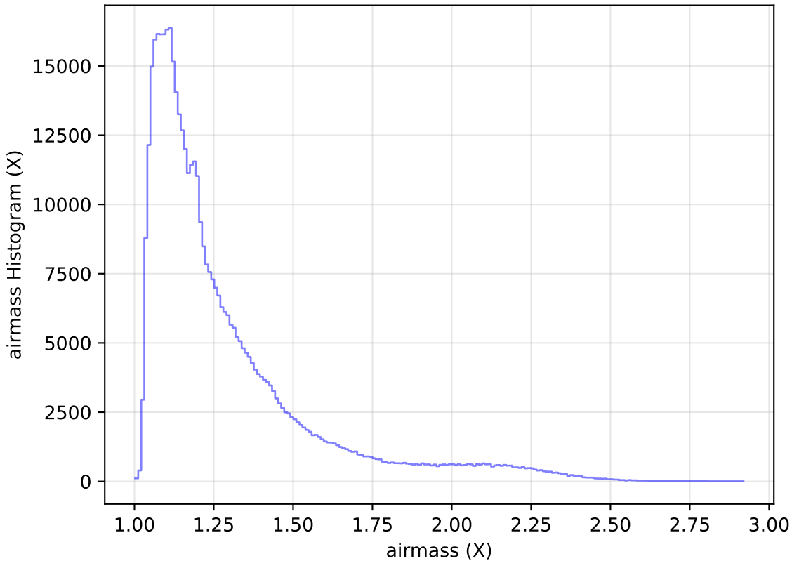
too_ignore_100_4v3.4_10yrs All sky r band: airmass Histogram
