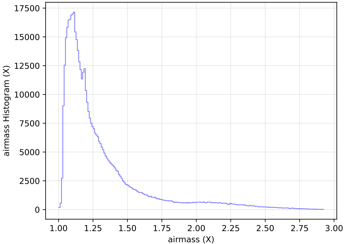
too_ignore_100_4v3.4_10yrs All sky i band: airmass Histogram
