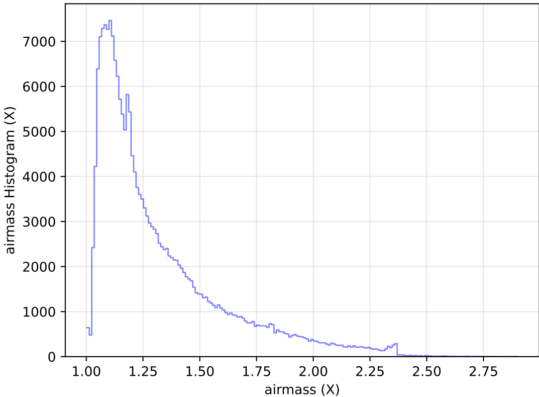
too_ignore_100_4v3.4_10yrs All sky g band: airmass Histogram
