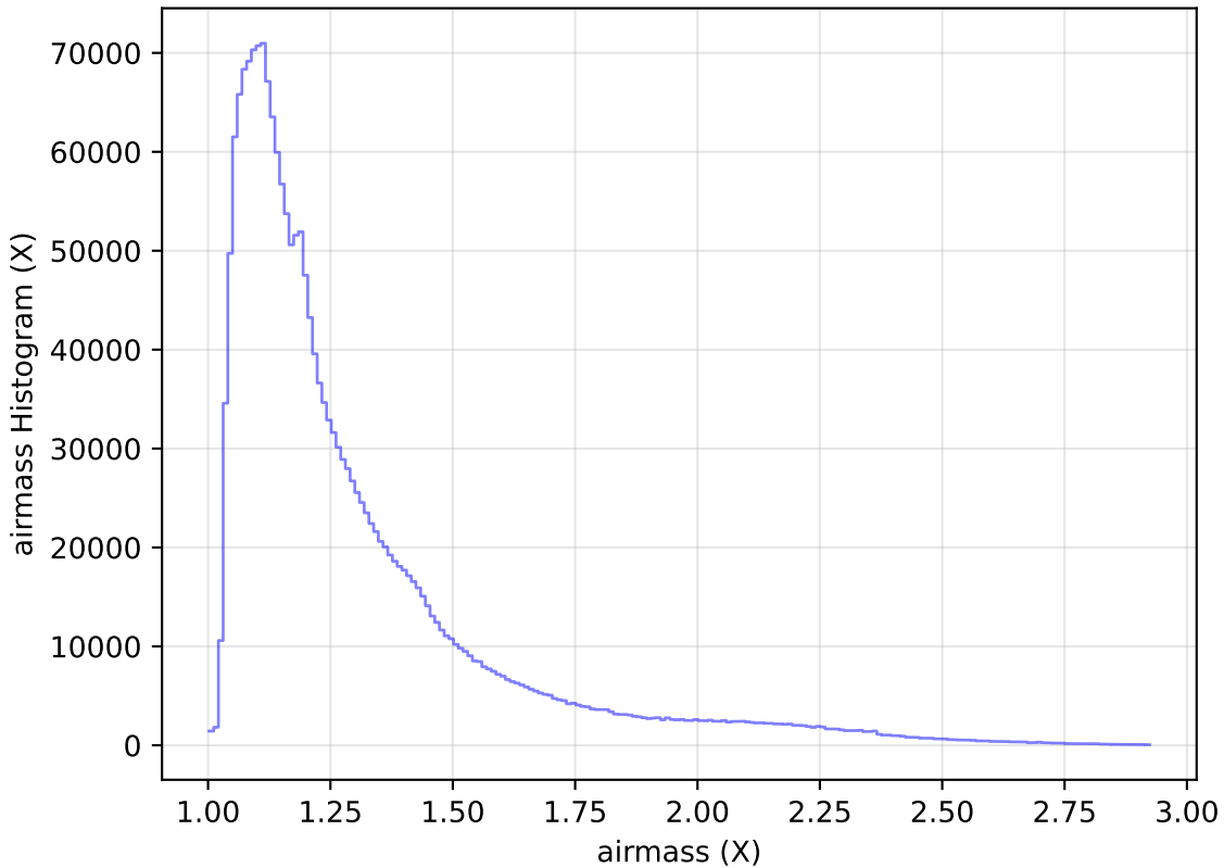
too_ignore_100_4v3.4_10yrs All sky all bands: airmass Histogram
