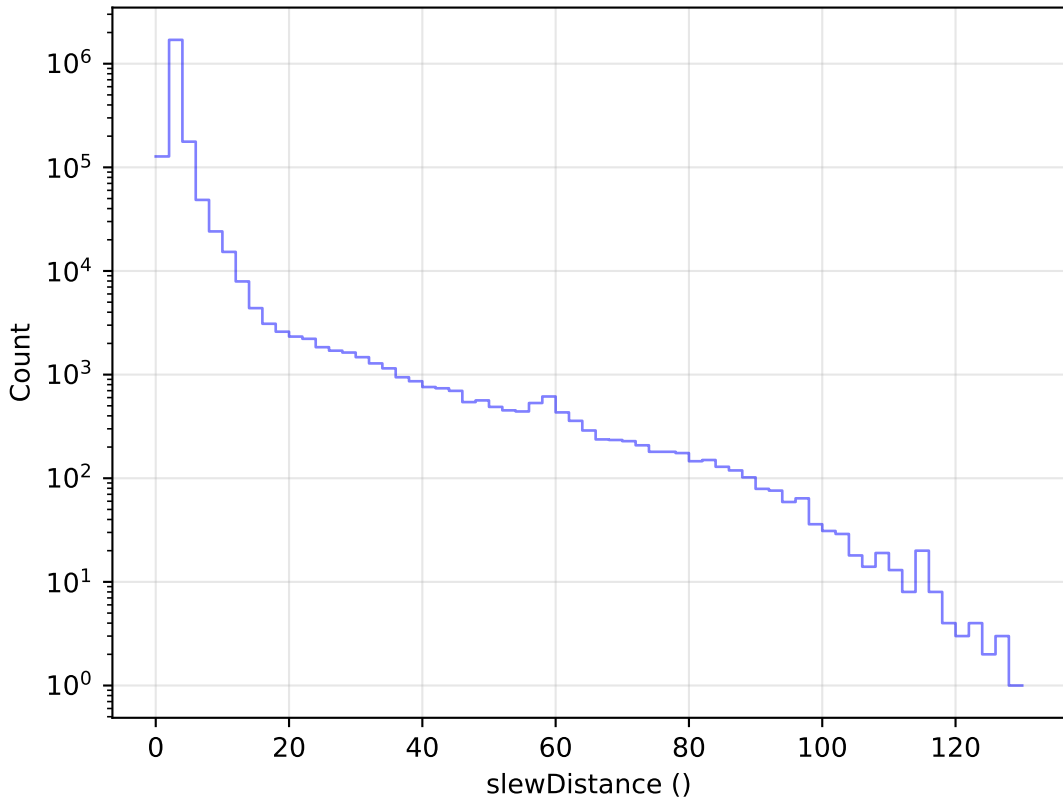
too_ignore_100_4v3.4_10yrs All visits: Slew Distance Histogram
