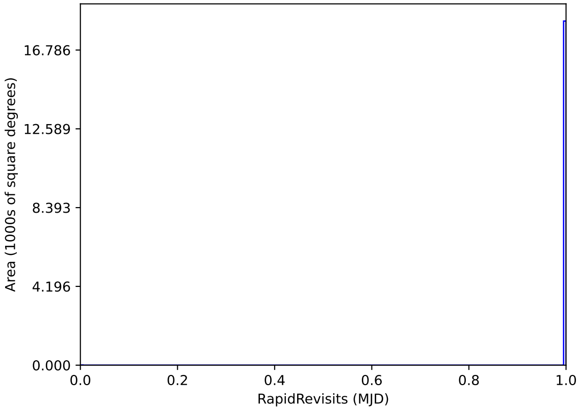
too_ignore_100_4v3.4_10yrs WFD: RapidRevisits
