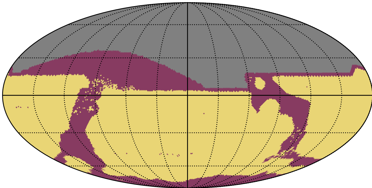
too_ignore_100_4v3.4_10yrs All sky: RapidRevisits
