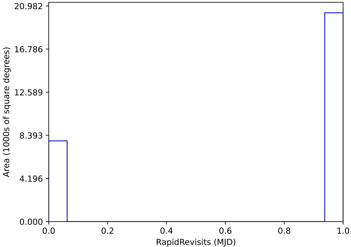
too_ignore_100_4v3.4_10yrs All sky: RapidRevisits
