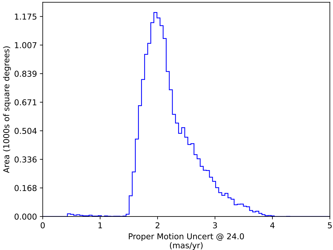
too_ignore_100_4v3.4_10yrs WFD: Proper Motion Uncert @ 24.0
