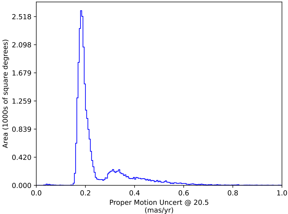
too_ignore_100_4v3.4_10yrs All sky: Proper Motion Uncert @ 20.5
