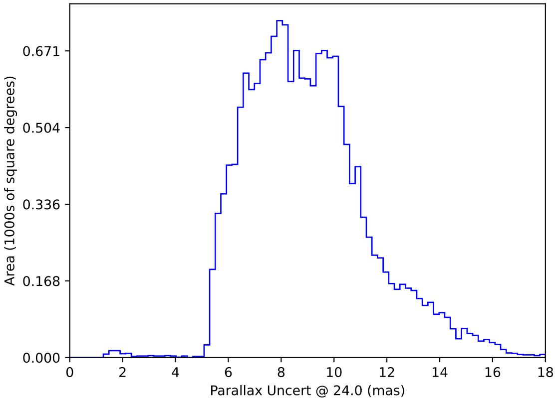
too_ignore_100_4v3.4_10yrs WFD: Parallax Uncert @ 24.0
