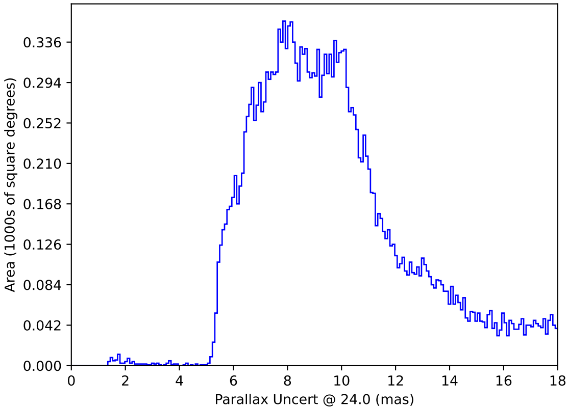
too_ignore_100_4v3.4_10yrs All sky: Parallax Uncert @ 24.0
