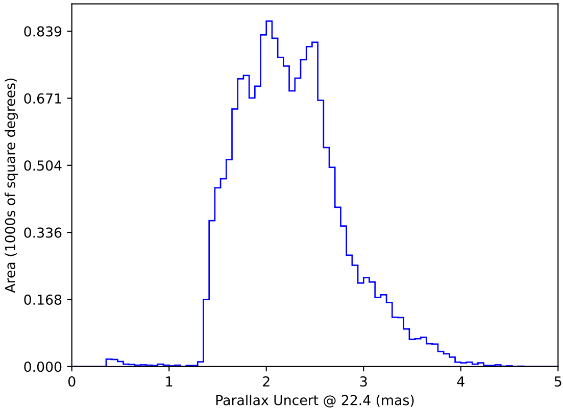
too_ignore_100_4v3.4_10yrs WFD: Parallax Uncert @ 22.4
