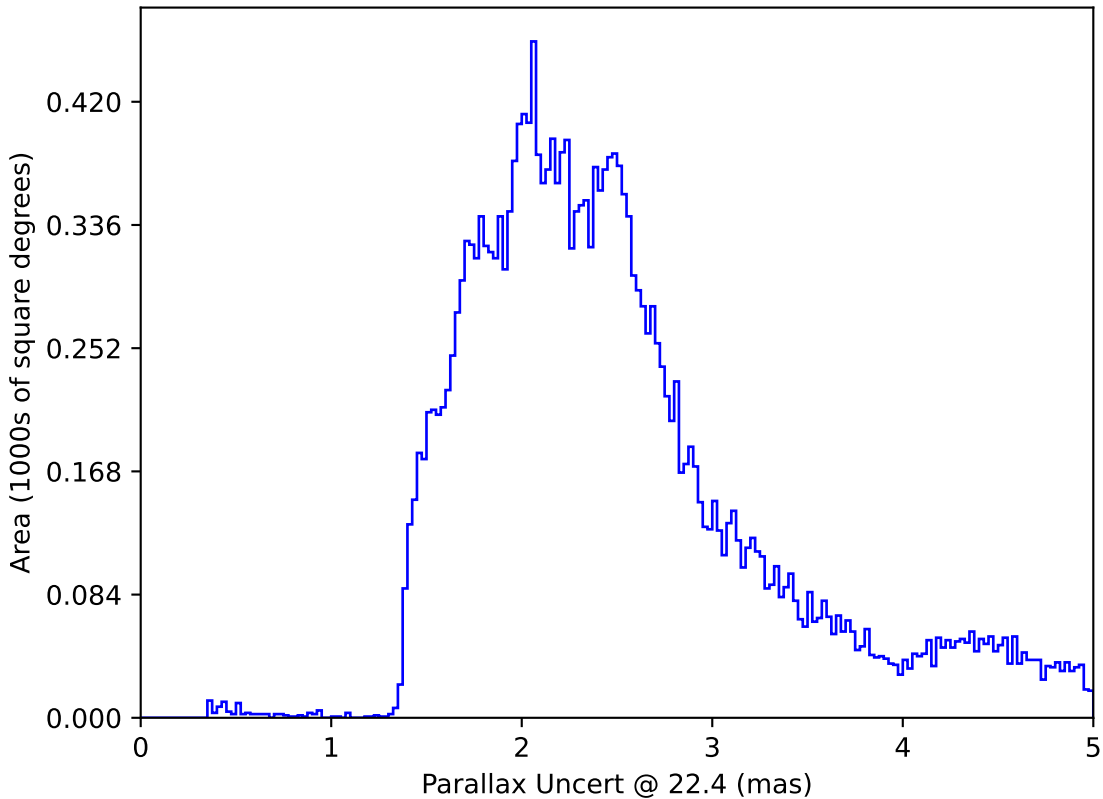
too_ignore_100_4v3.4_10yrs All sky: Parallax Uncert @ 22.4
