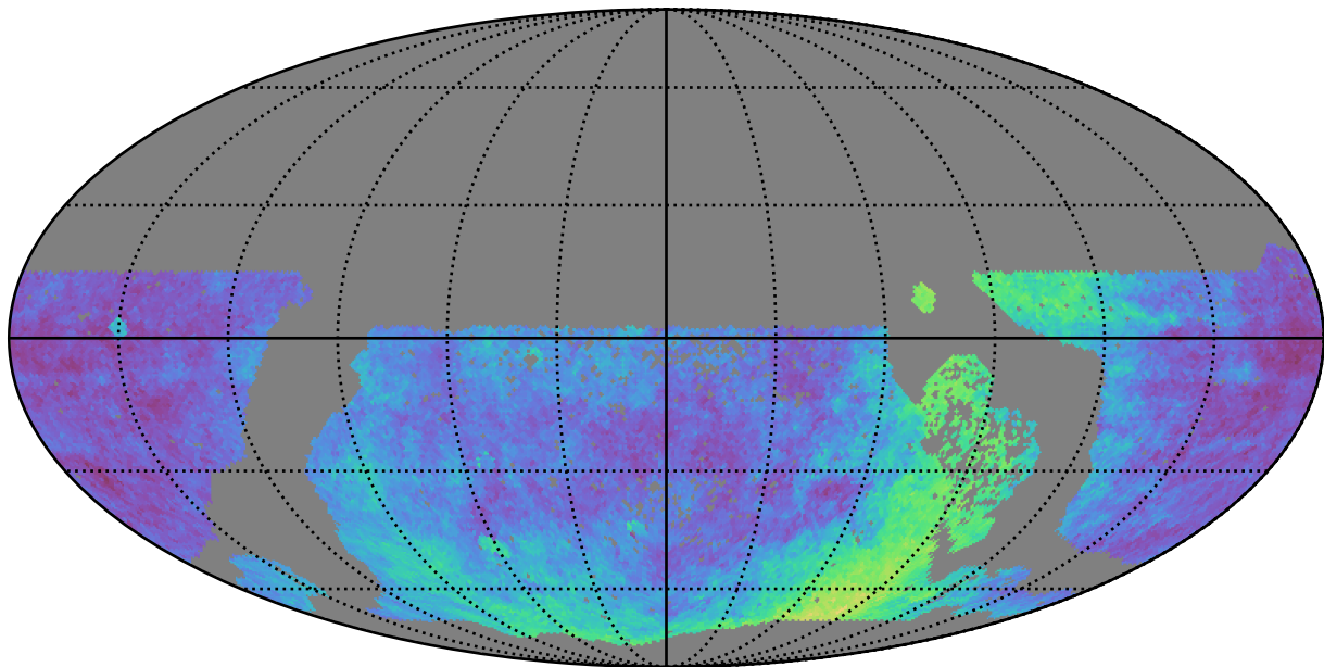
too_ignore_100_4v3.4_10yrs WFD: Parallax Coverage @ 24.0
