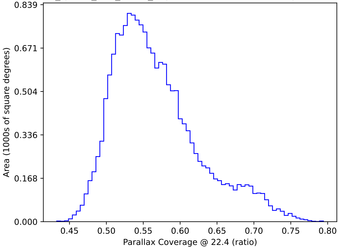
too_ignore_100_4v3.4_10yrs WFD: Parallax Coverage @ 22.4
