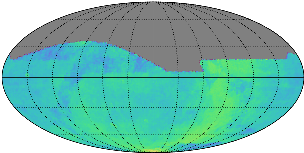
too_ignore_100_4v3.4_10yrs All sky: Parallax Coverage @ 22.4
