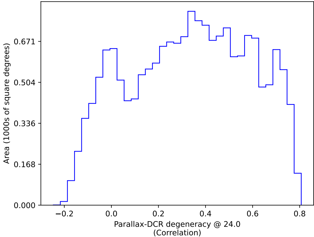
too_ignore_100_4v3.4_10yrs WFD: Parallax-DCR degeneracy @ 24.0
