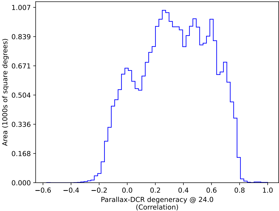
too_ignore_100_4v3.4_10yrs All sky: Parallax-DCR degeneracy @ 24.0
