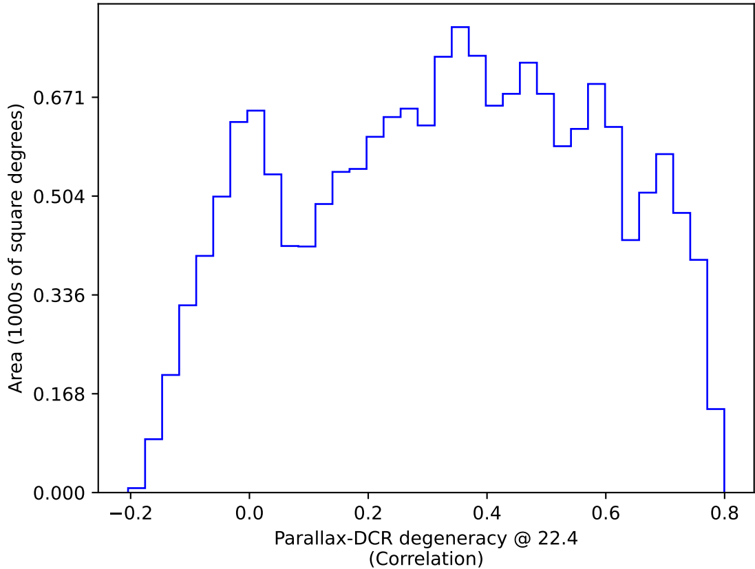
too_ignore_100_4v3.4_10yrs WFD: Parallax-DCR degeneracy @ 22.4
