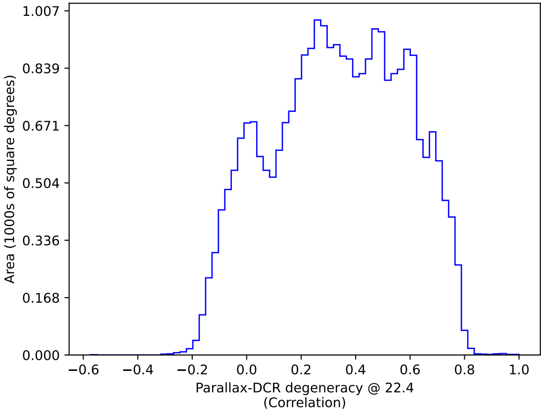
too_ignore_100_4v3.4_10yrs All sky: Parallax-DCR degeneracy @ 22.4
