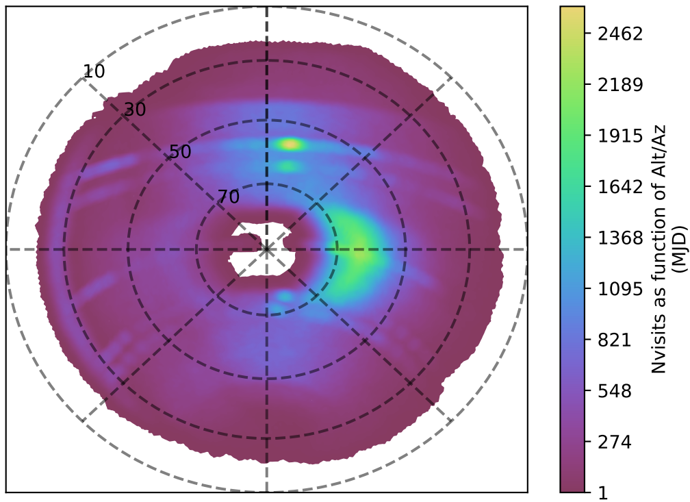
too_ignore_100_4v3.4_10yrs r band: Nvisits as function of Alt/Az
