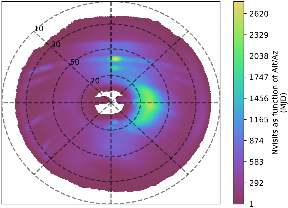
too_ignore_100_4v3.4_10yrs i band: Nvisits as function of Alt/Az
