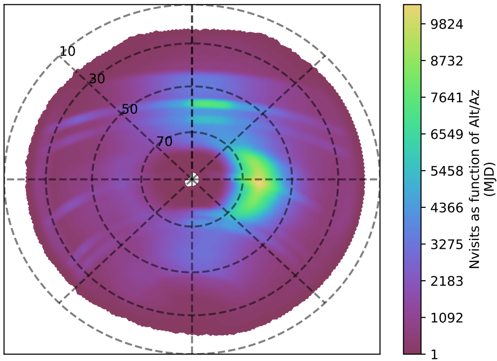
too_ignore_100_4v3.4_10yrs all bands: Nvisits as function of Alt/Az
