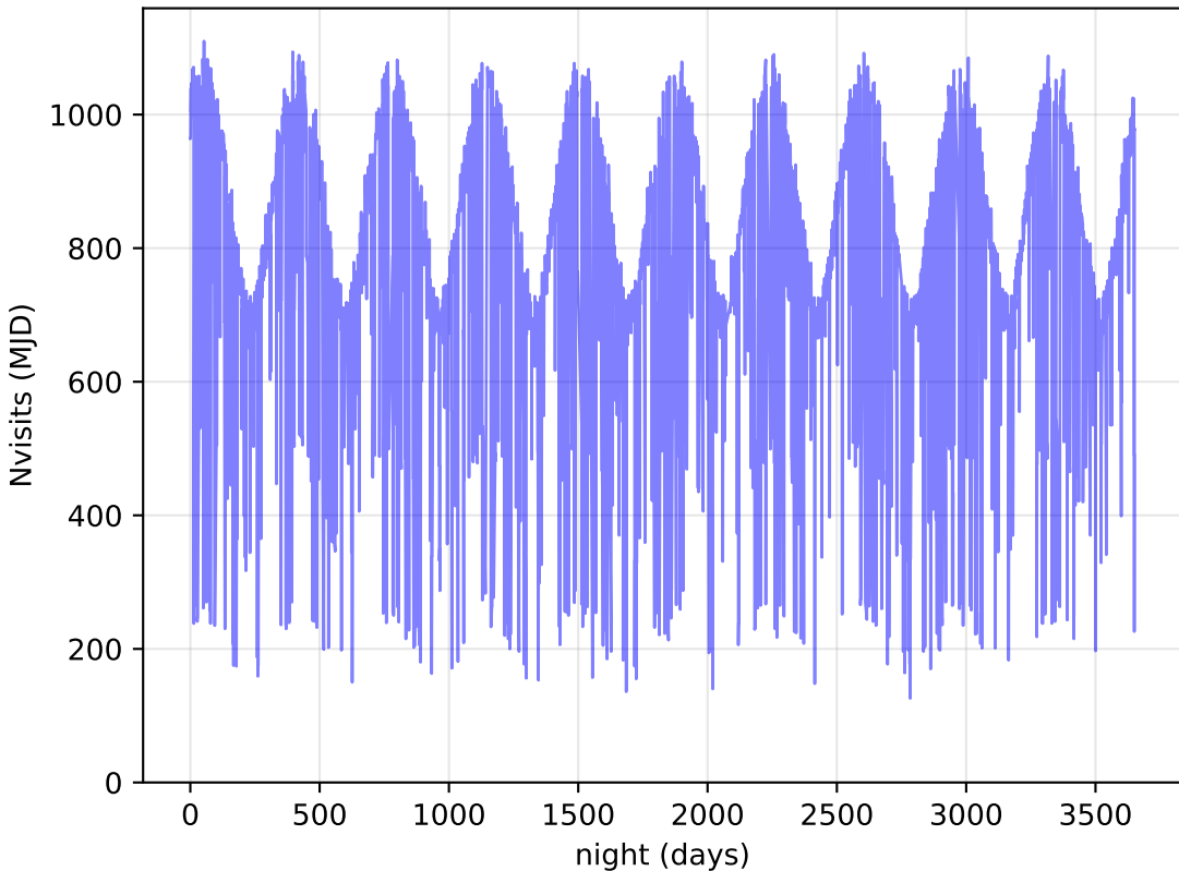
too_ignore_100_4v3.4_10yrs All visits: Nvisits
