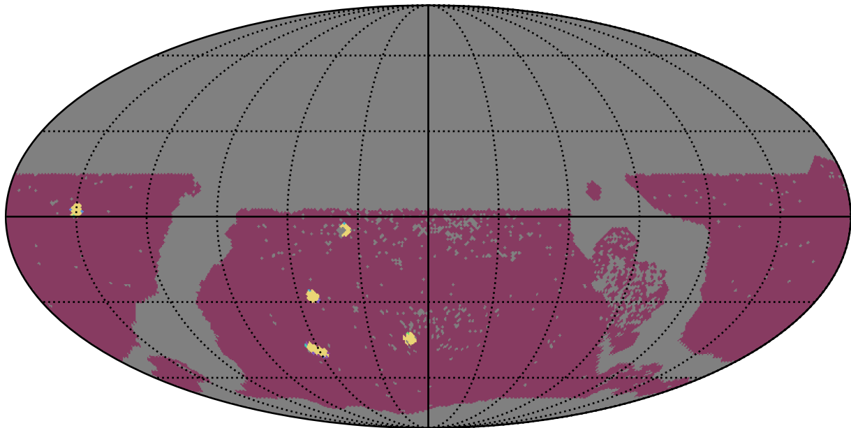
too_ignore_100_4v3.4_10yrs WFD: NumberOfQuickRevisits
