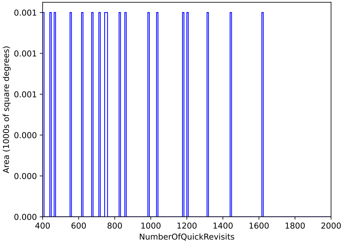
too_ignore_100_4v3.4_10yrs WFD: NumberOfQuickRevisits
